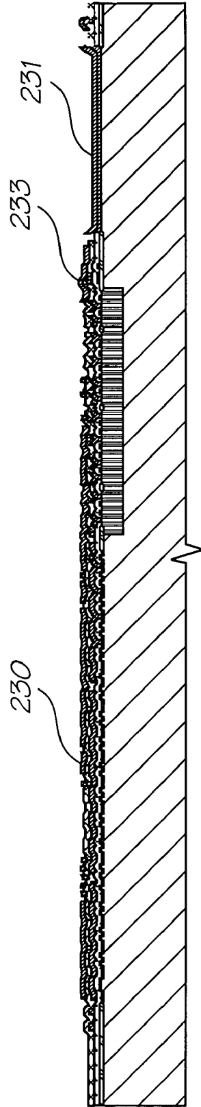
Deposit metal 2
